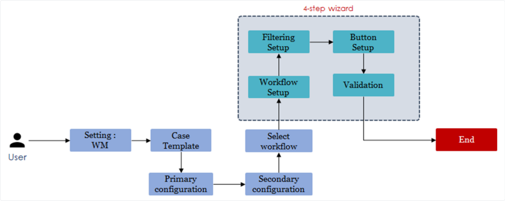
Figure 2.1: Watchlist - Case Template
